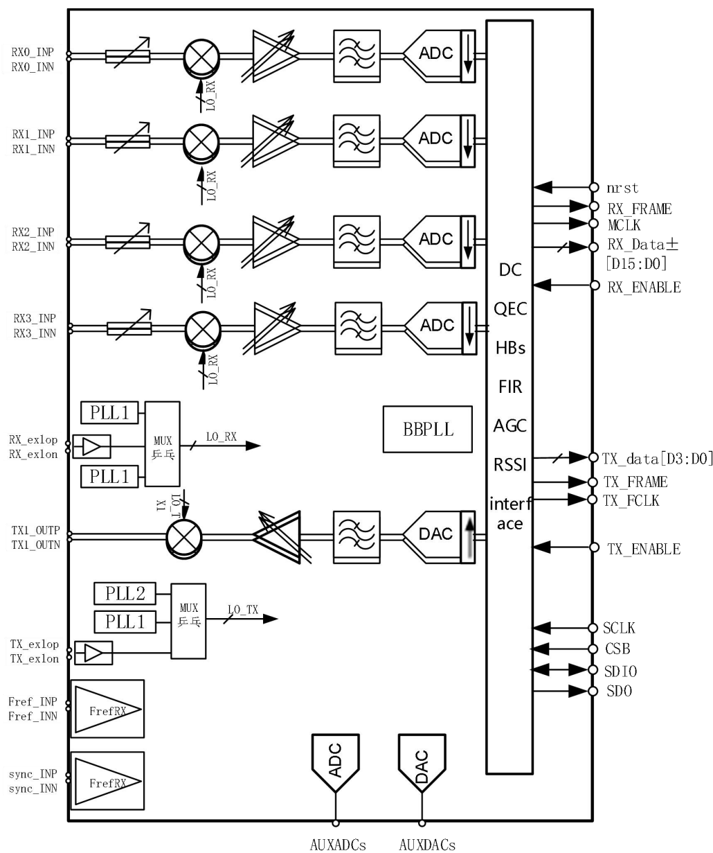
CX9450S/CX9450SN 功能框图
